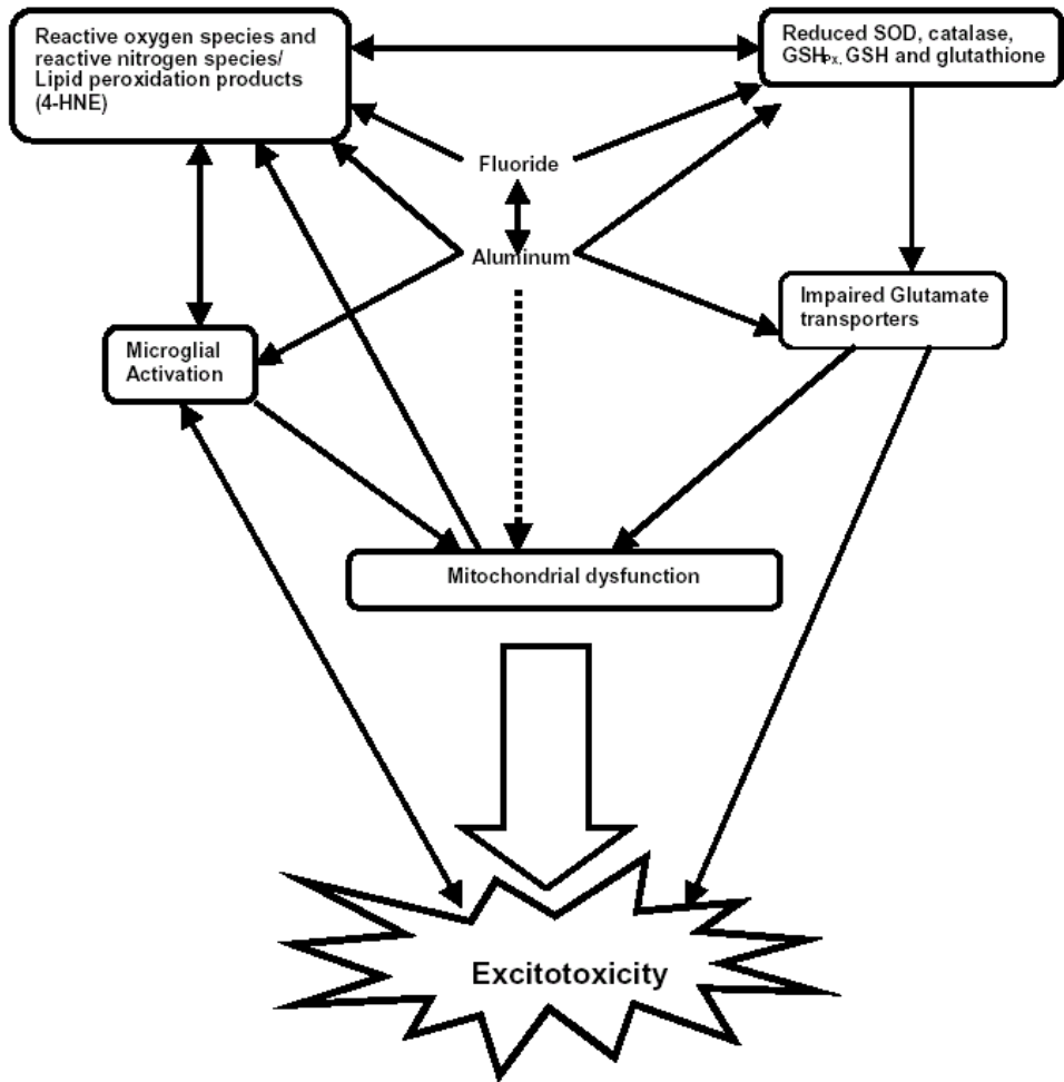
Figure. Possible mechanisms for neurodegenerative effects of fluoride and aluminum as related to excitotoxicity. The broken arrow represents the effects of both elements.
