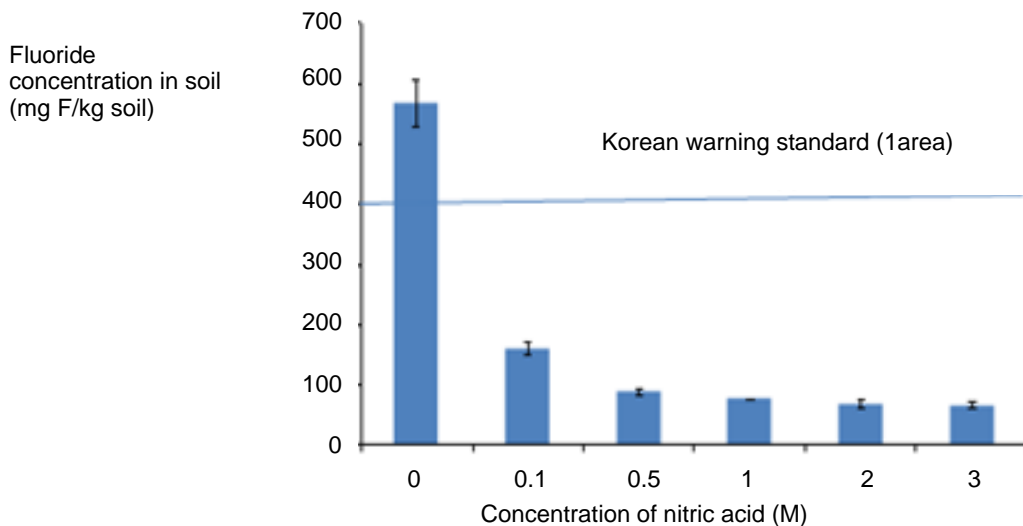
Figure 10. Fluoride concentrations remaining in the soil after nitric acid (HNO 3 ) washing at various concentrations together with the Korean warning standard for one area. 31
